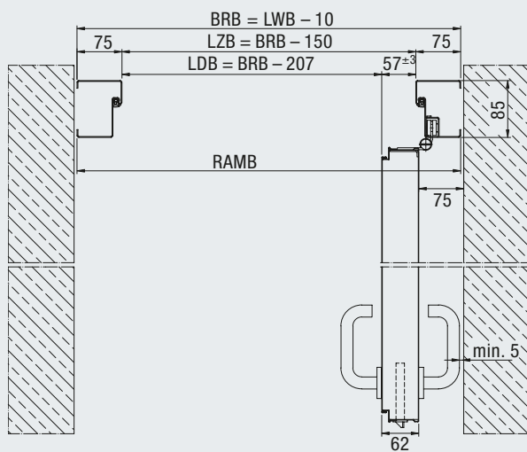
Blockzarge 95 / 55 (STS)
