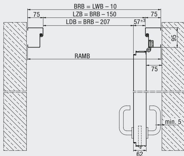
Blockzarge 105 / 100 (STS)
