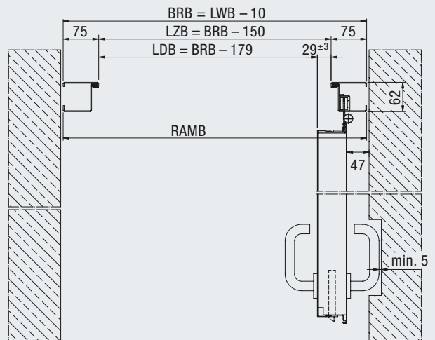
Blockzarge 62 / 75 (STU)
