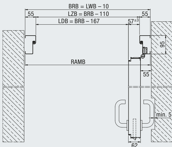
Blockzarge 95 / 55 (STS)
