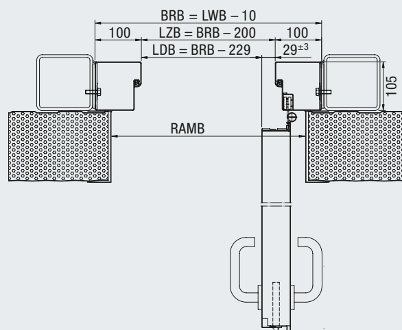
Blockzarge 105 / 100 (STU) Hallenbau-Paneelwand
