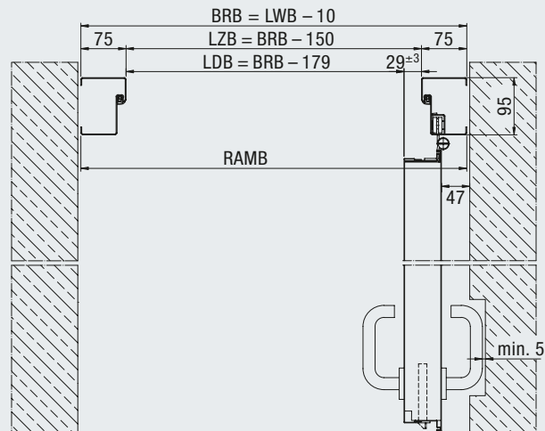
Blockzarge 105 / 100 (STU)
