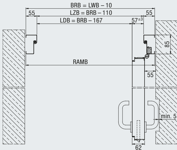
Blockzarge 85 / 75 (STS)
