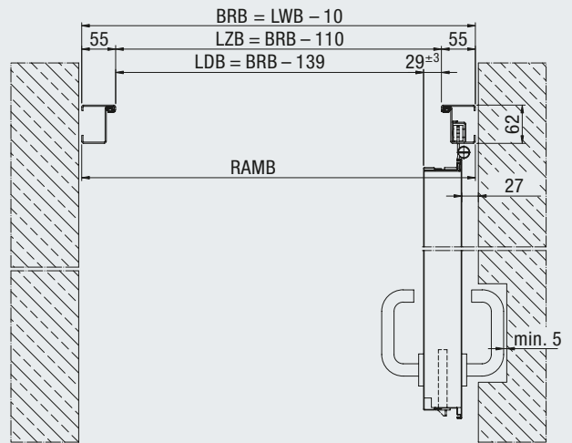
Blockzarge 62 / 75 (STU)
