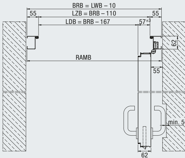
Blockzarge 62 / 75 (STS)
